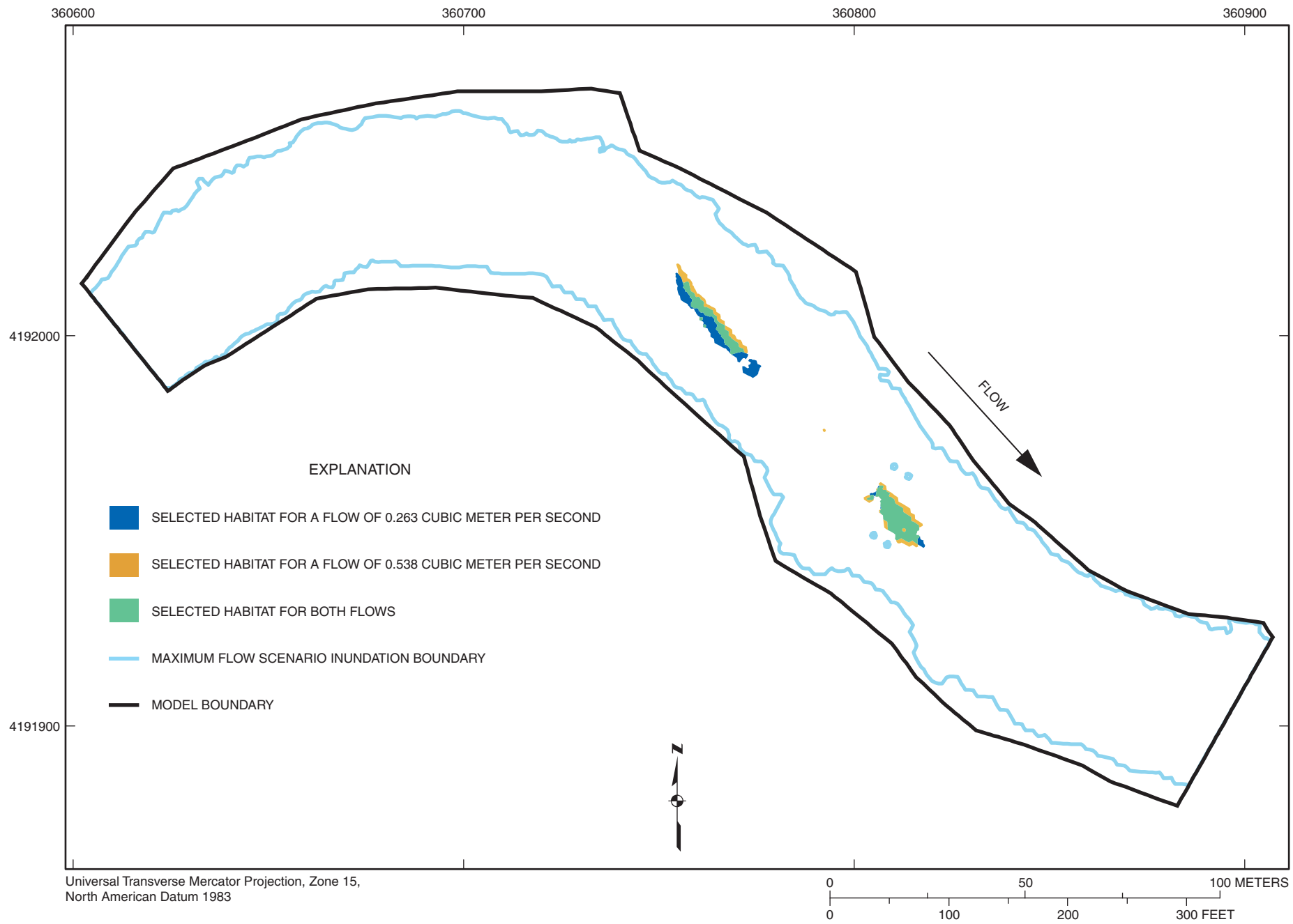
Figure 1-39. Selected habitat area distribution for habitat category 19 (stonecat) at flows of 0.263 and 0.538 cubic meter per second at Marmaton River site M1.
